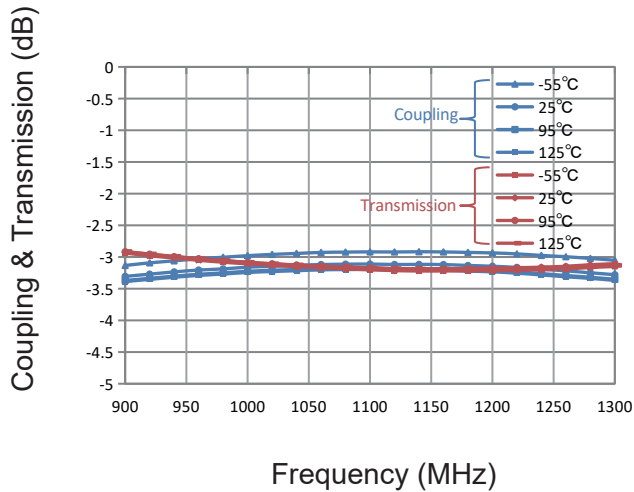
Coupling & Transmission (Port 1 feeding)
