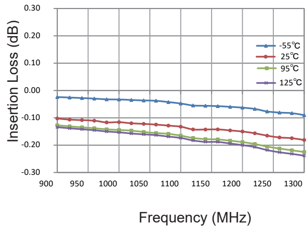
Insertion Loss (Port 1 feeding)
