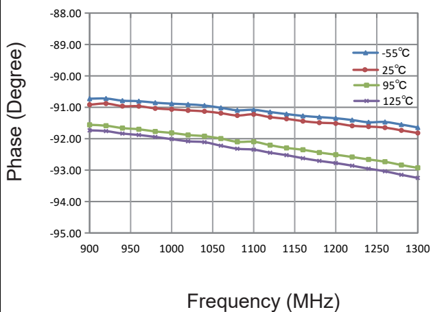
Phase (Port 1 feeding)
