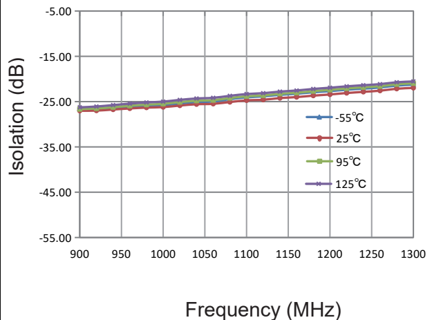
Isolation (Port 1 feeding)
